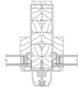
VERTICAL MULLION
