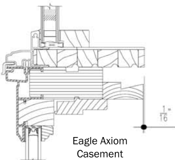
HORIZONTAL MULLION
