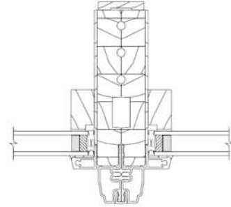
VERTICAL MULLION
