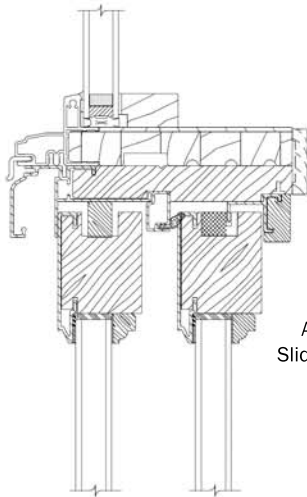
HORIZONTAL MULLION
