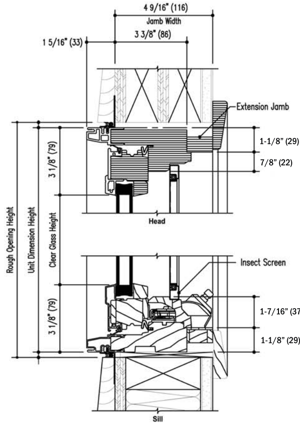
Vertical Section
