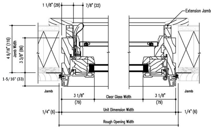
Horizontal Section
